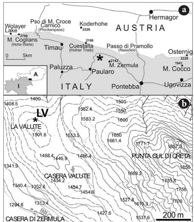
Fig. 1 - Location map. a) Schematic map of the Carnic region, with location of the La Valute area (asterisk). b) Topographic map of the western part of Mt. Zermula massif, with location of the La Valute section.
